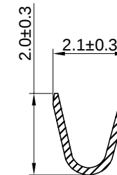
SEC B-B
