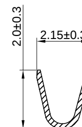
SEC B-B
