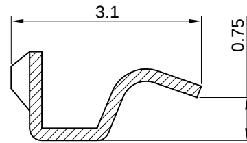
SEC B-B
